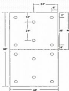
Fastener Drawing Pattern
